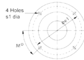
Sizes K03 to K08
