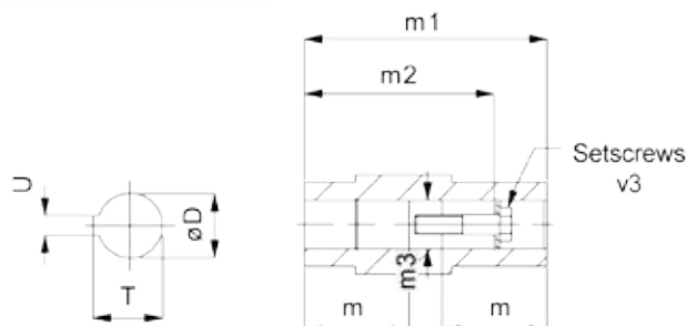
Output Shaft Bore
