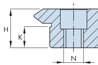
Tapped Hole Option N
