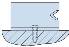
Blind Fixing Flanged Type
