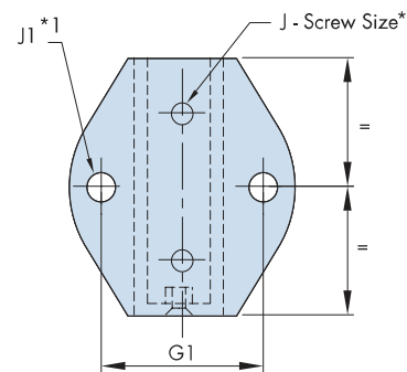
Option - FB*3 For use with Floating Bearings
