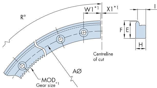
External Single Edge Track Segment - TRE
