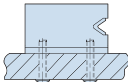
Through Fixing Compact Type
