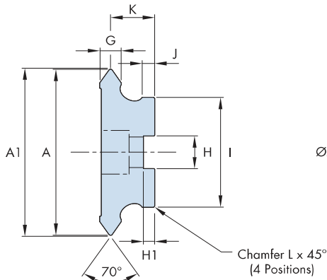
Dowel Pin 3 (SDP)
