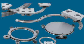
PRT2 Precision Ring and Track System
