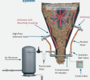
Standard AirSweep™ System
