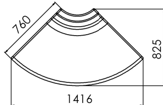
90° External corner High Back
