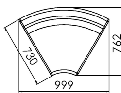
60° Internal corner Low Back
