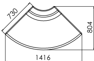
90° External corner Low Back
