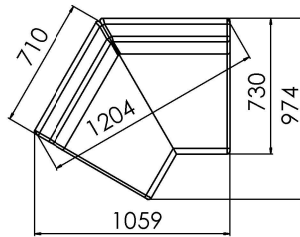
60° Internal 710W corner Low Back
