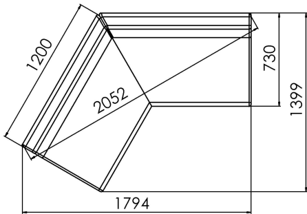
60° Internal 1200W corner Low Back
