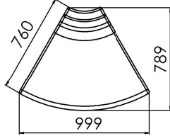
60° External corner High Back
