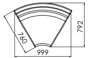
60° Internal corner High Back
