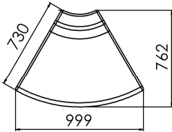
60° External corner Low Back
