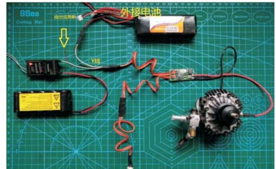
Receiver power supply connection diagram
