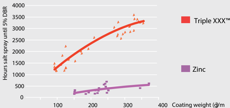
Corrosion resistance of standard galv wire and Triple XXX™ in salt spray environment 5% DBR - Results on wire level
