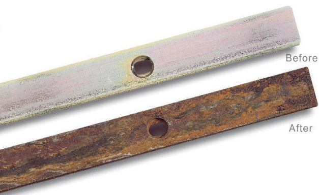
3,000 hours Salt Spray Test Stainless Steel
