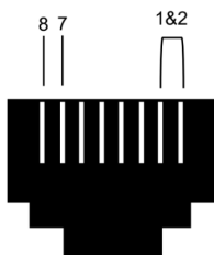
RJ45 Connection
