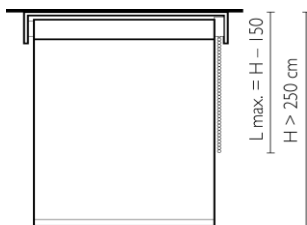
CHAIN LENGTH
