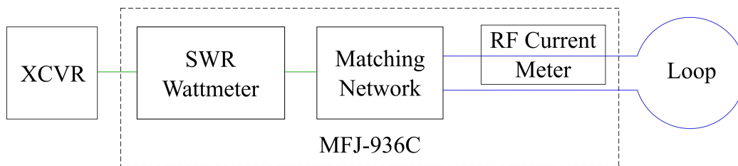
Figure 6: Typical MFJ-936C Configuration
