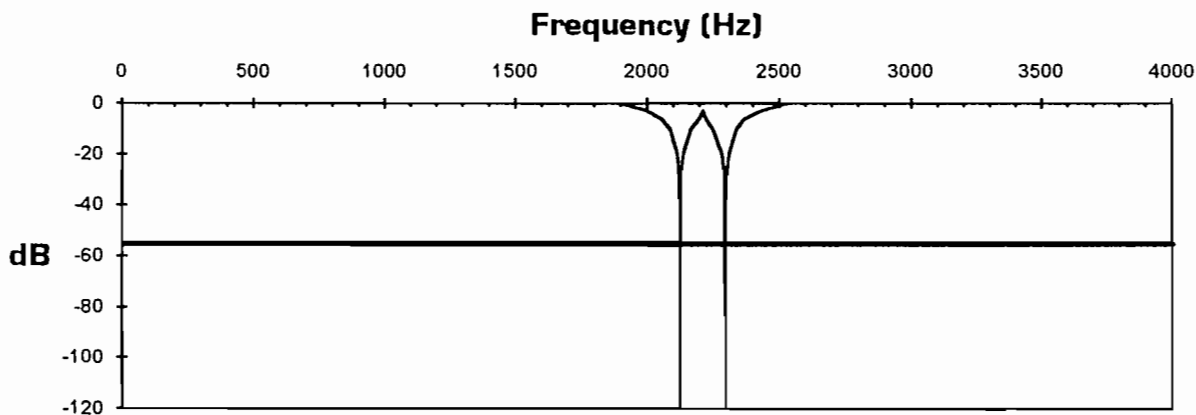
Typical Manual Notch Filter Response
