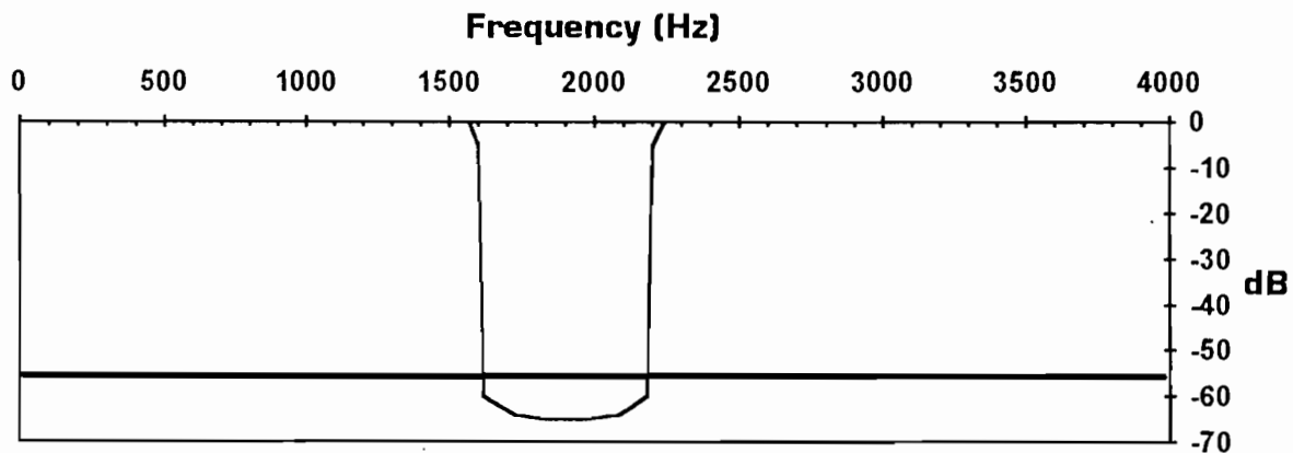
Typical Band-stop Filter Response
