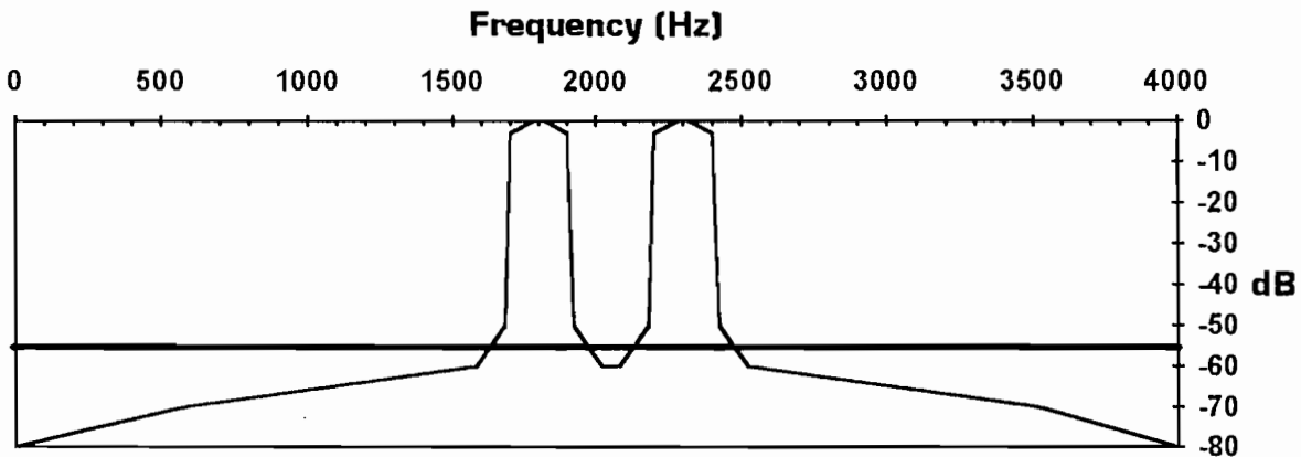
Typical Dual Band-pass Filter Response
