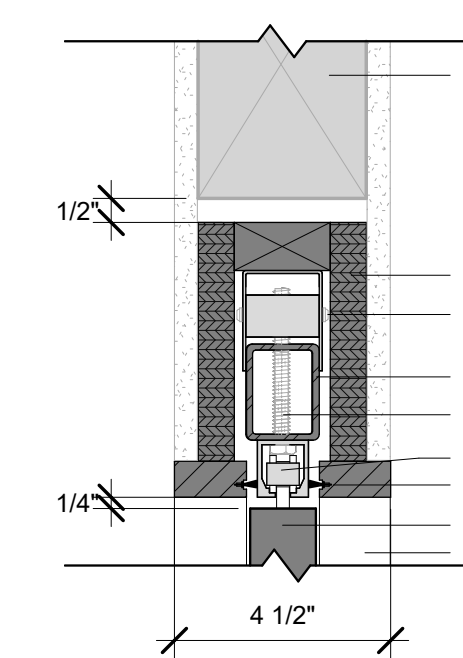
⑦ PPDS Section Detail 3" 1'-0"
