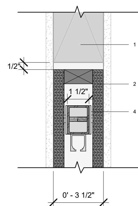
④ Enlarged Section 3" 1'-0"
