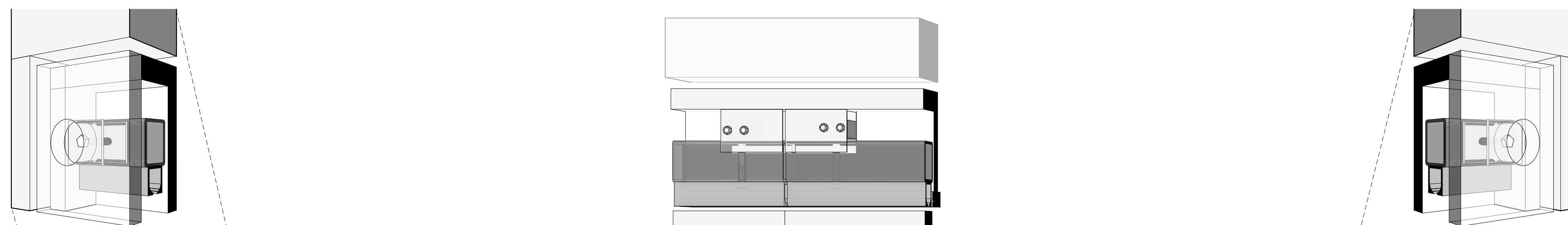
⑤ Pocket Door Assembly - Horizontal Section 1 1/2" 1'-0"
