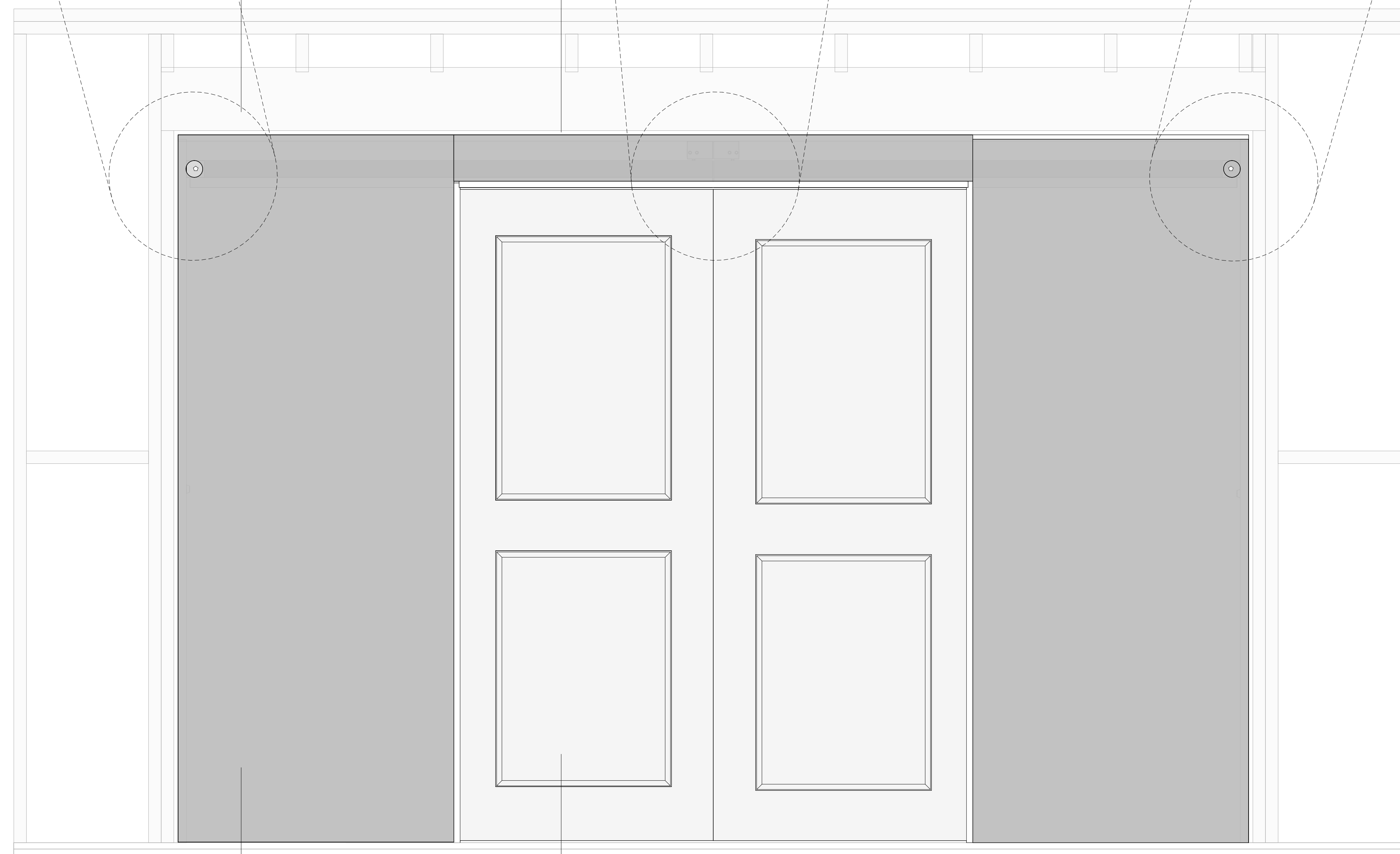
② Pocket Door Assembly Elevation 1 1/2" 1'-0"
