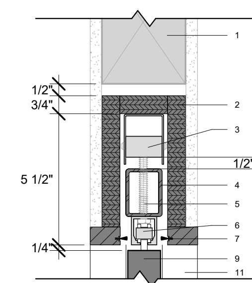
⑦ PPDS Section Detail 3" 1'-0"
