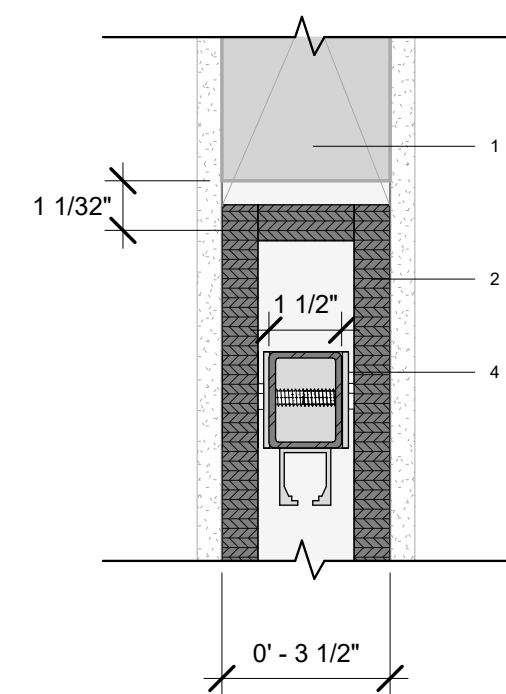
④ Enlarged Section 3" 1'-0"
