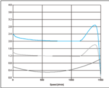
A sample taken from the MotSize dimensioning program showing DOL starting curves for a cast iron motor:
