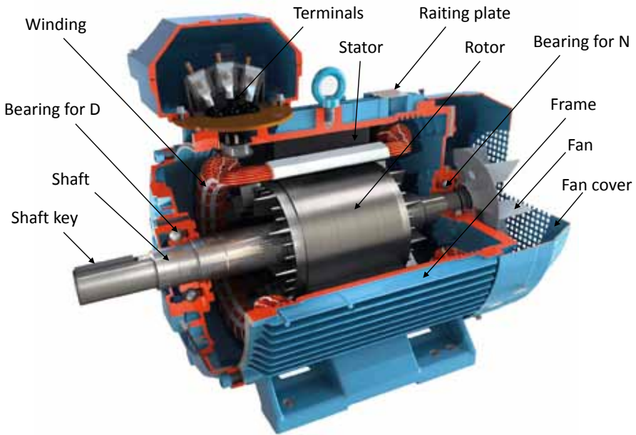
Figure 5.1 Cross-section of a cast-iron induction motor
