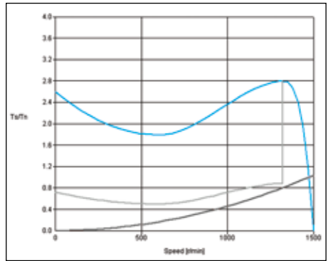
A sample taken from the MotSize dimensioning program showing Y/Δ starting curves for an aluminum motor:
