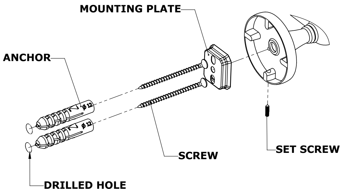
DETAIL M
