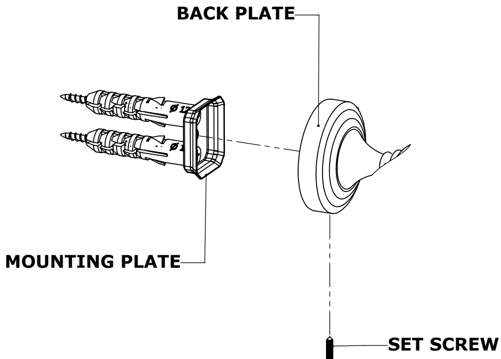
DETAIL N
