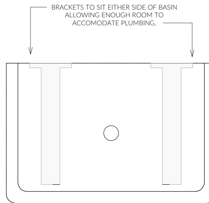
UNDERSIDDE OF POD w/ BRACKET POSITION
