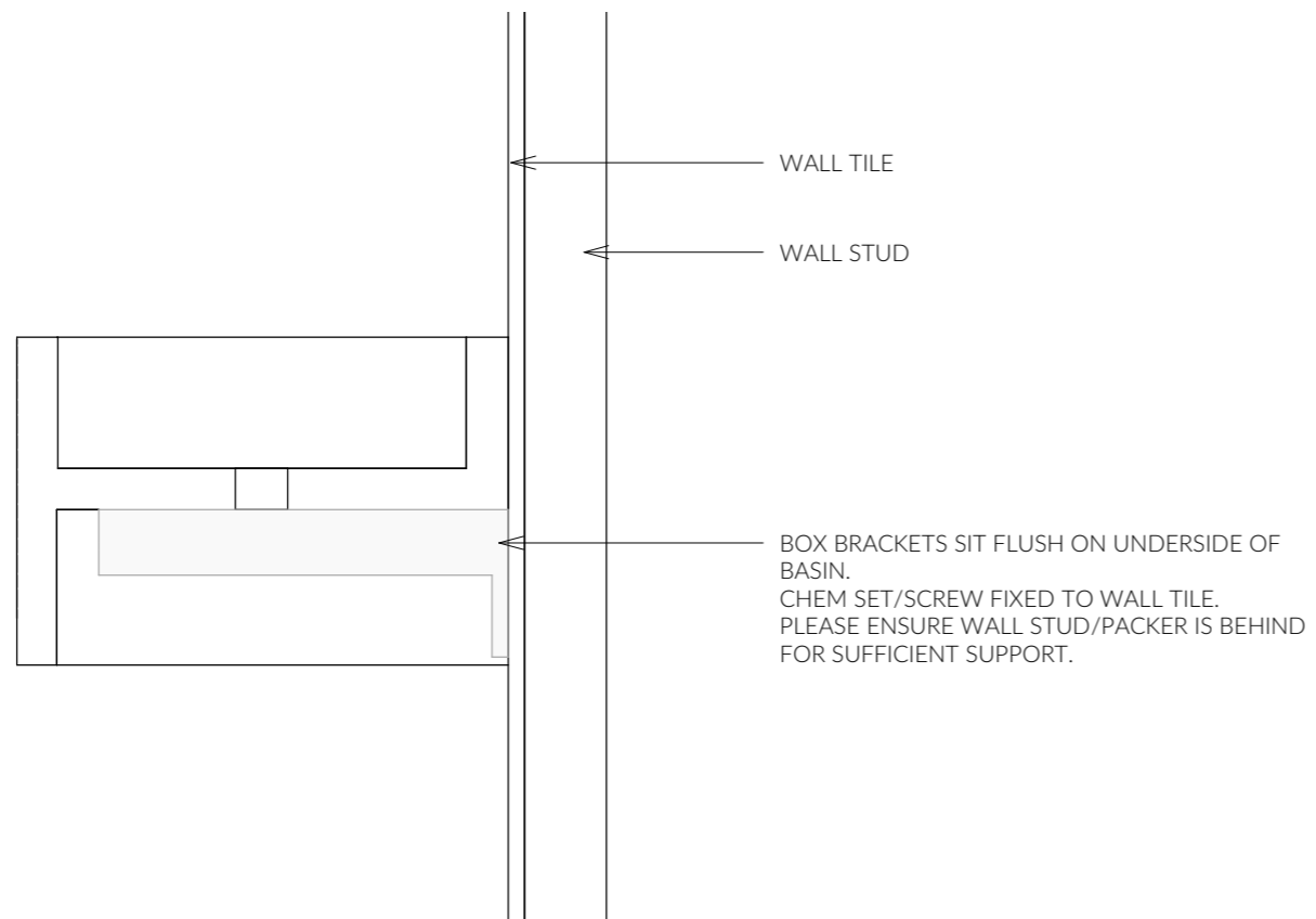
SECTION OF POD w/ BRACKET POSITION TO WALL
