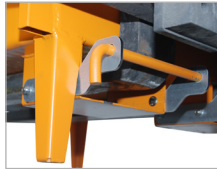
Secured by bolt to prevent slipping from the forklift truck
