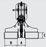
Fork sleeve inside dimensions in mm
