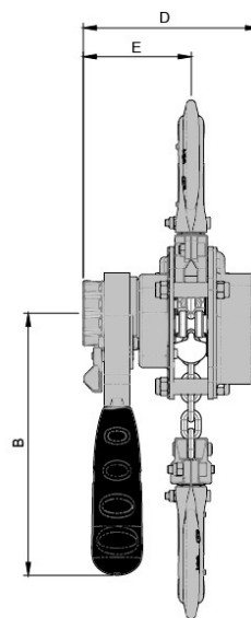
0.5t lever hoist (LH-0050)
