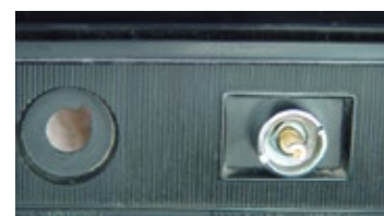
Photo 24. This photo shows the later 1969 -74 Delay Switch and installation hardware. Your switch may look different, depending on the year of your car and type of switch.
