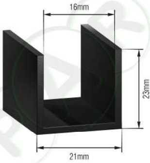
PR1330 U-Channel
