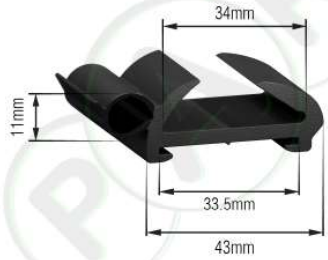
PR612 EPDM Caravan Window Frame Seal
