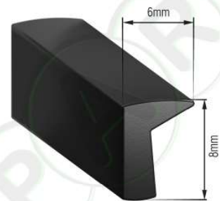
PR149 EPDM Ghia Seal
