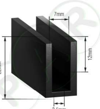
PR1213 Square U Channel EPDM
