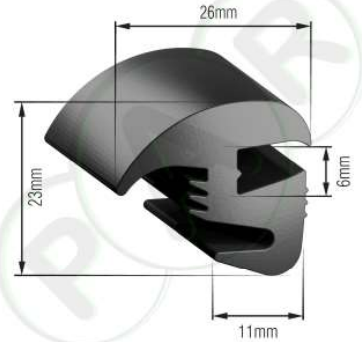
PR212 Universal S-Type Windscreen Profile
