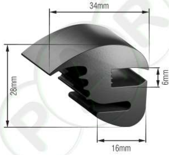
PR210 Windscreen Rubber: Ford Cortina, Ford F250
