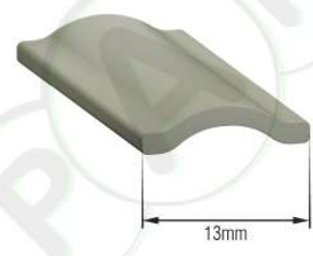
PR491W PVC Thick Aluminium Trim White
