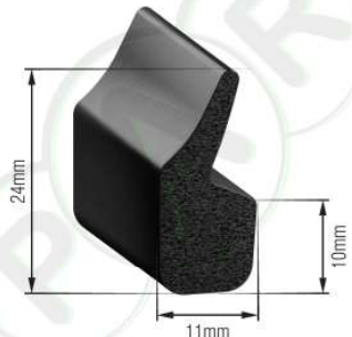
PR311 EPDM/Sponge Universal door seal for VW Beetle, Kombi, Merc Bulnose
