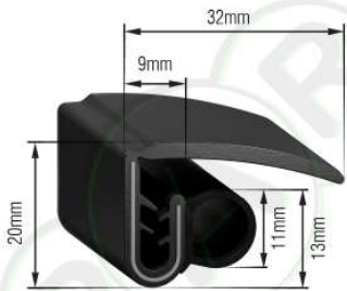
PR602 EPDM/Sponge 20mm Doorseal
