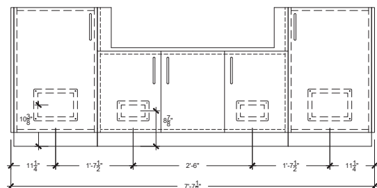
FRONT VIEW (Gas & Electrical Conduits Access Points)
