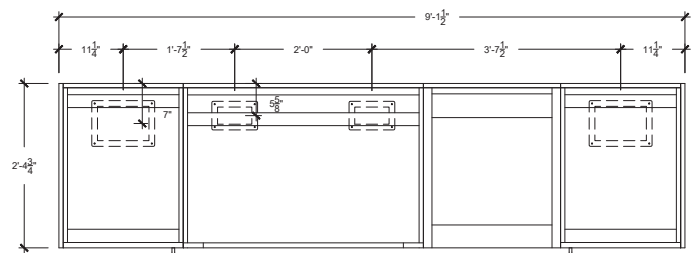
FRONT VIEW (Gas & Electrical Conduits Access Points)
