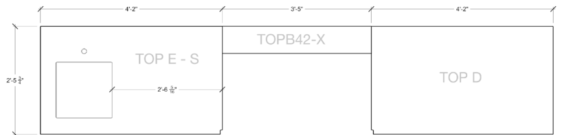
COUNTERTOP TEMPLATE
