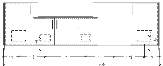
FRONT VIEW (Gas & Electrical Conduits Access Points)
