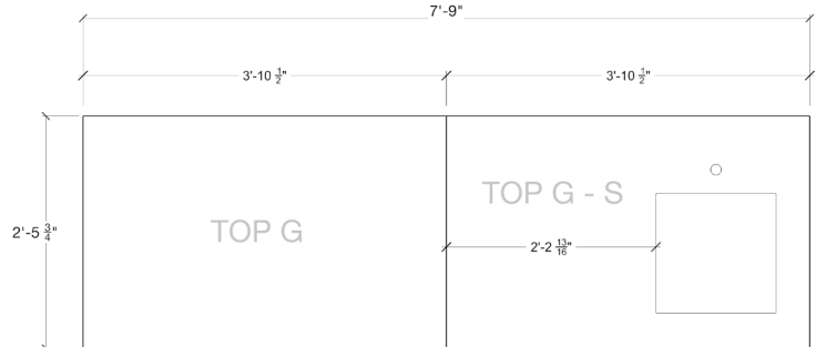
COUNTERTOP TEMPLATE
