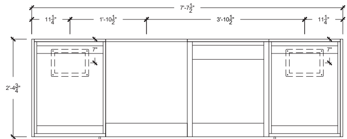
TOP VIEW (Gas & Electrical Conduits Access Points)
