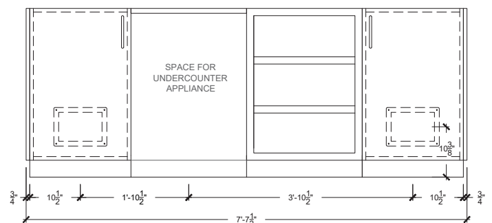
FRONT VIEW (Gas & Electrical Conduits Access Points)
