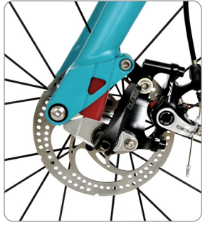
FRONT FORK UPGRADE KIT (includes PU and 140mm disc rotor)
