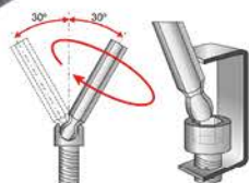
The ball end allows misalignment of up to 30° for use in tight spaces
