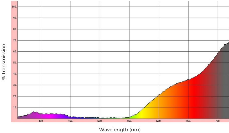
Spectrophotometry Graph
