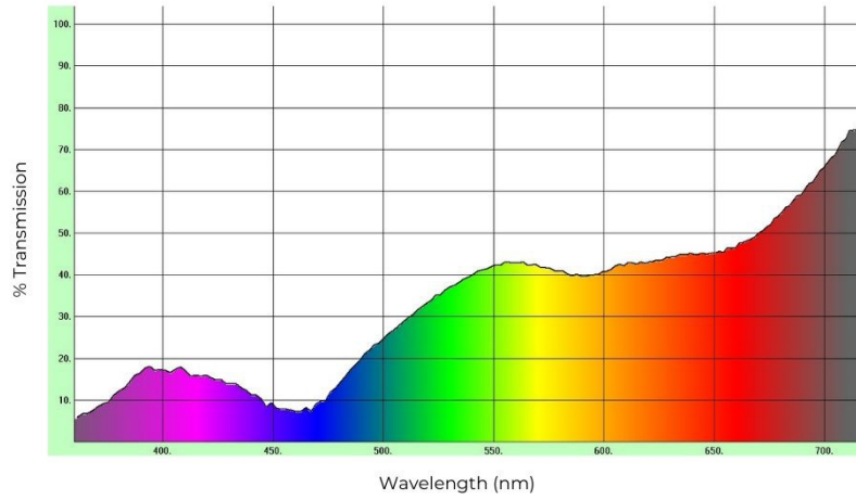
Spectrophotometry Graph
