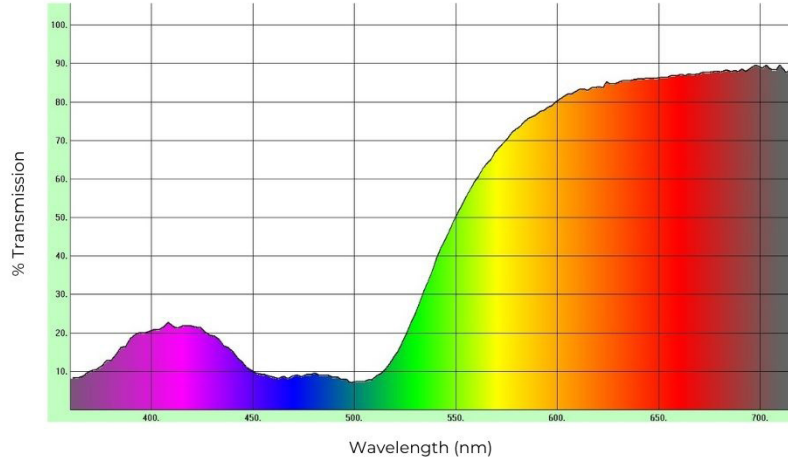
Spectrophotometry Graph
