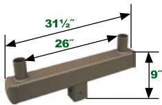
5 Twin Square Vertical Tenon NHL-BH5-2180-SQ Wt lbs 29.25, EPA 1.0
