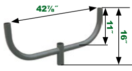
180° Double Bullhorn NHL-BH-180 Wt lbs 17, EPA 0.9
