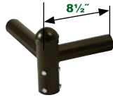
Twin Spoke Bracket, 90° Arms NHL-RSF-290
