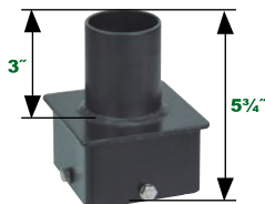
5 Single Square Vertical Tenon - 2 3/8" Dia. NHL-SSF5-2.7/8
