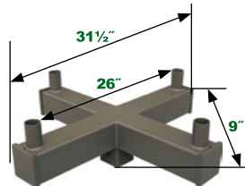
5 90° Quad Square Vertical Tenon NHL-BH5-490-SQ Wt lbs 49, EPA 1.1
