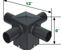
4" 90° Quad Square Horizontal Tenon NHL-SSF4-490
