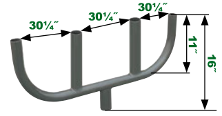
180° Quad Bullhorn NHL-BH4-180 Wt lbs 38, EPA 2.2
