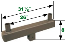
4" Twin Square Vertical Tenon NHL-BH4-2180-SQ Wt lbs 25, EPA 1.0
