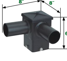
4" 90° Twin Square Horizontal Tenon NHL-SSF4-290
