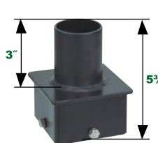
4" Single Square Vertical Tenon - 2 1/2" Dia. NHL-SSF4-2.7/8
