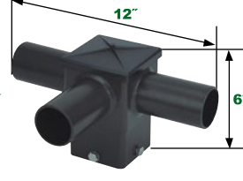
4" 90° Triple Square Horizontal Tenon NHL-SSF4-390
