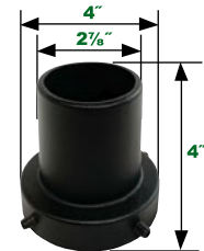
Retrofit Tenon Adaptor for 2 3/8" Tenons NHL-PTA-2/3
