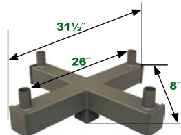
4" 90° Quad Square Vertical Tenon NHL-BH4-90-SQ Wt lbs 44, EPA 1.1
