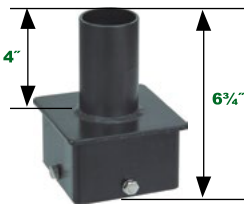
4" Single Square Vertical Tenon - 2 3/8" Dia. NHL-SSF4-2.3/8
