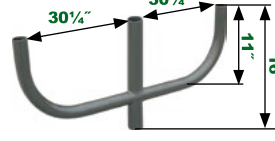
180° Triple Bullhorn NHL-BH3-180 Wt lbs 27, EPA 1.5
