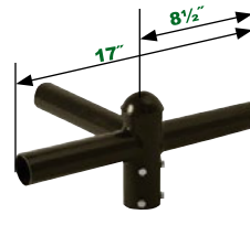
Triple Spoke Bracket, 90° Arms NHL-RSF-390*
