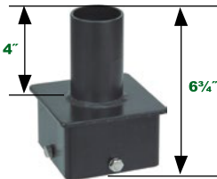
5 Single Square Vertical Tenon - 2 3/8" Dia. NHL-SSF5-2.3/8
