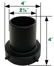
Retrofit Tenon Adaptor for 2 3/8" Tenons NHL-PTA-2/3
