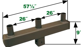
5 Triple Square Vertical Tenon NHL-BH5-3180-SQ Wt lbs 46, EPA 1.9
