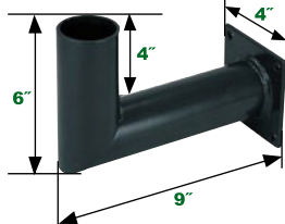
Wall Mount 90° Bracket NHL-WMB90 Wt lbs 4.5, EPA 0.3
