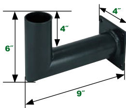
Wall Mount 90° Bracket NHL-WMB90
