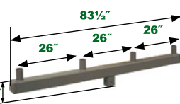
4. 180° Quad Square Vertical Tenon NHL-BH4-180-SQ Wt lbs 56, EPA 2.7
