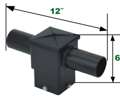
4" 180° Twin Square Horizontal Tenon NHL-SSF4-2180
