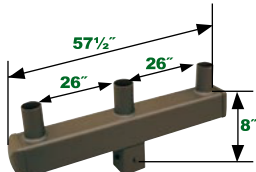
4" Triple Square Vertical Tenon NHL-BH4-3180-SQ Wt lbs 40, EPA 1.9
