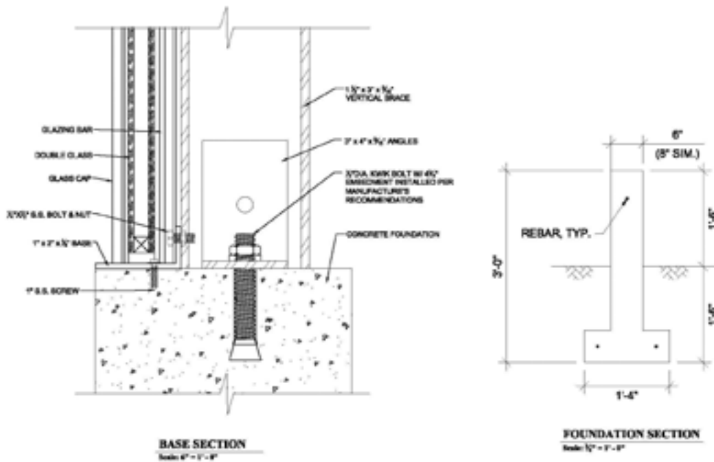
Dimensions and rebar are for reference only. Actual dimensions to be determined by local building code.
