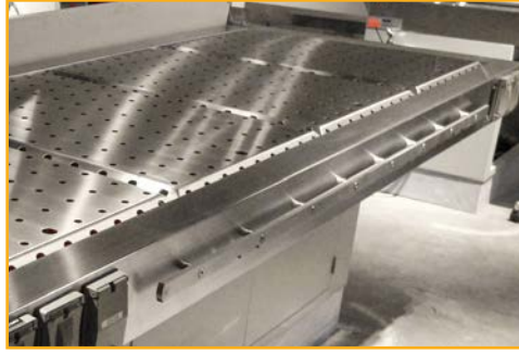
OA-502 - TIE DOWN BARS
