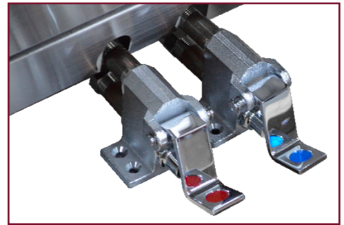
OA-151 - HOT AND COLD FOOT VALVE Sturdily constructed hot/cold foot pedal helps temper water and keep your hands free while working.
