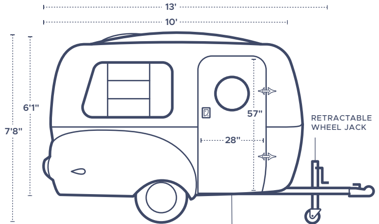
RIGID FRAME W/ TORSION AXLE & GWR OF 3500 LBS.
