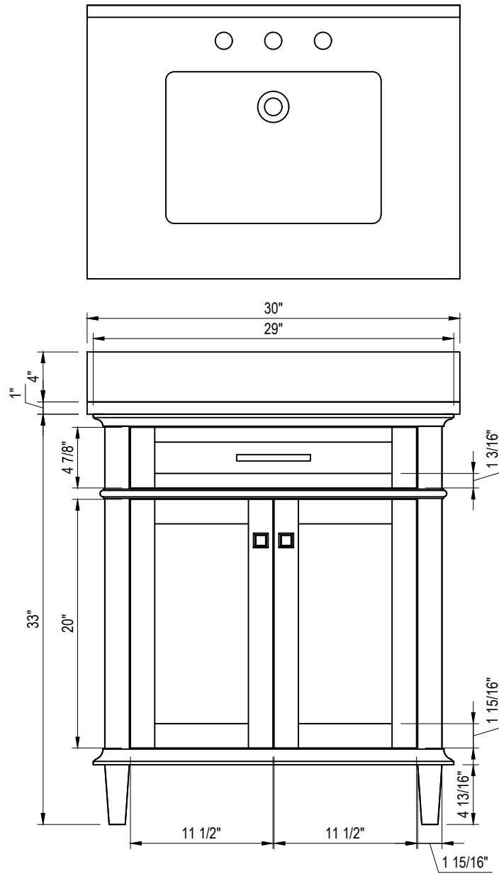
Front View
