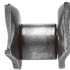
③ Offset link plate fatigue Offset link plates are bent at the center, and the resulting concentration of stress at the bend can cause a fatigue break. Avoid using offset links in high-stress applications.
