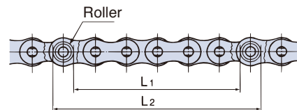
Fig. 28 Measuring length
