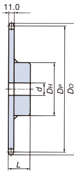
(Machined specifications) 1B type
