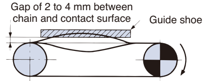
Fig. 21 Guide shoe to prevent vibration
