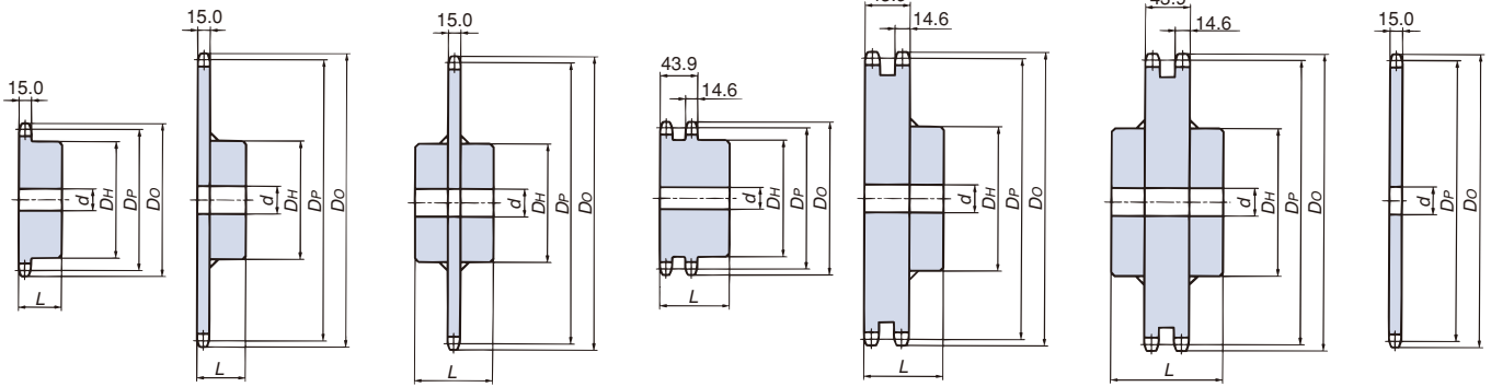
Mechanically machined 1B type, Welded construction 1B type, Welded construction 1C type, Mechanically machined 2B type, Welded construction 2B type, Welded construction 2C type, 1A type
