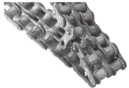
Fig. 31 Corrosion of stainless steel roller chain
