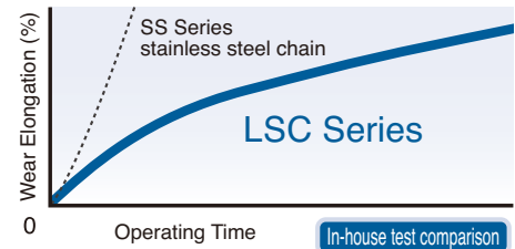
Wear life comparison with stainless steel chain (18-8 stainless steel, SUS304 equiv.)
