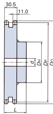
(Machined specifications) 2B type
