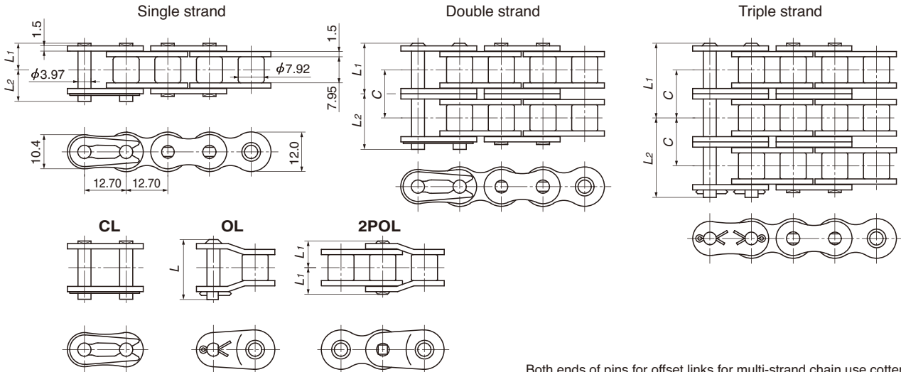
Both ends of pins for offset links for multi-strand chain use cotter pins.
