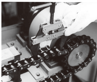
Fig. 9 Connecting between shafts
