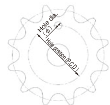
Hanging hole dimensions
