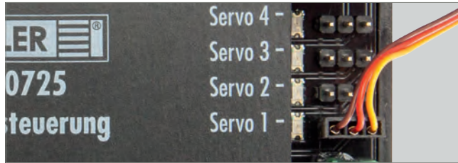
Fig. 3: Connecting servos
