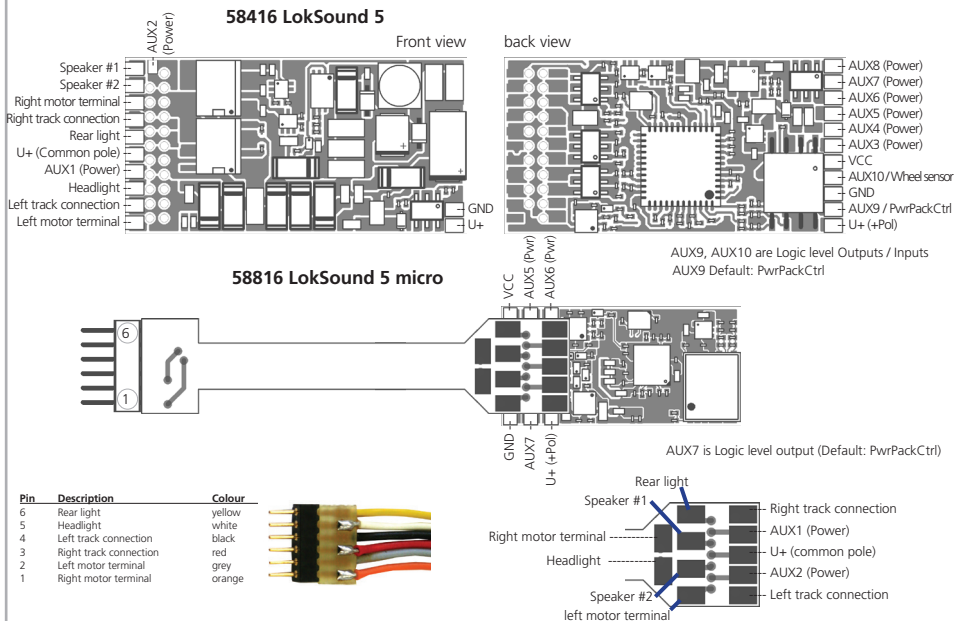
Figure 2: LokSound 5 & LokSound 5 micro with 6-pin NEM651 Interface
