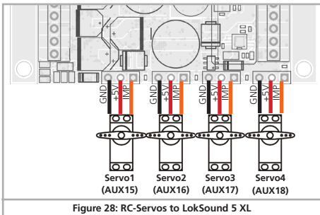
Figure 28: RC-Servos to LokSound 5 XL
