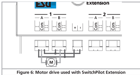
Figure 6: Motor drive used with SwitchPilot Extension
