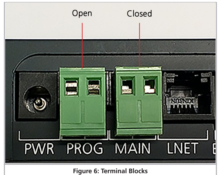
Figure 6: Terminal Blocks
