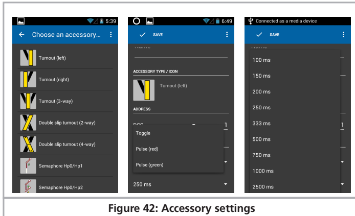
Figure 42: Accessory settings
