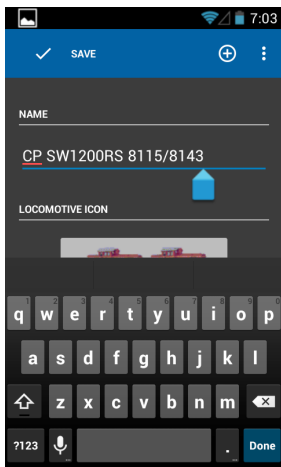
Figure 36: Name consist
