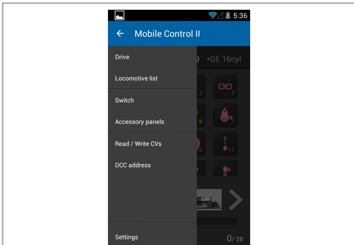
Figure 19: Main menu
