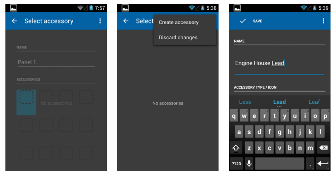
Figure 41: Create Accessory
