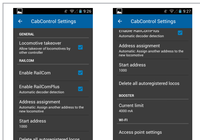
Figure 52: CabControl Settings
