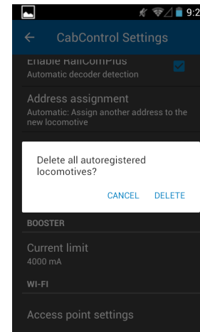
Figure 55: Delete all
