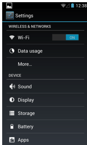
Figure 9: Set-up menu
