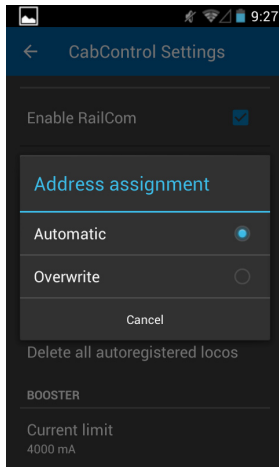
Figure 53: Address Assignment
