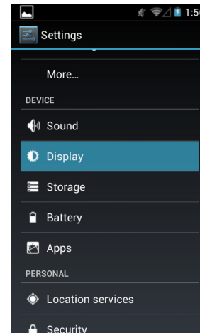
Figure 11: Display settings
