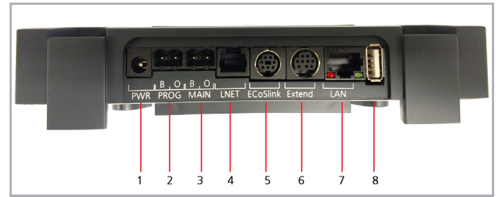
Figure 4: Integrated Control Unit Back
