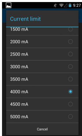
Figure 56: Current limit
