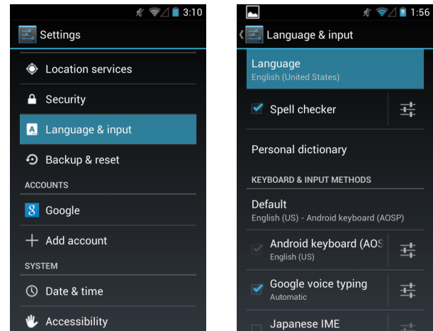
Figure 10: Language settings
