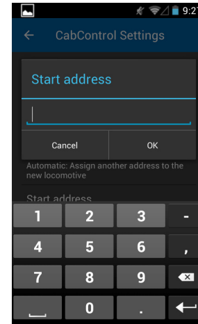
Figure 54: Start Address
