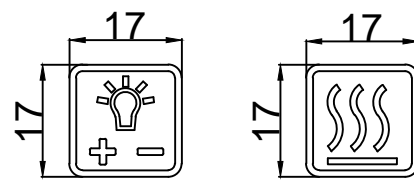
按键激光镂空 Keystroke laser hollow out
