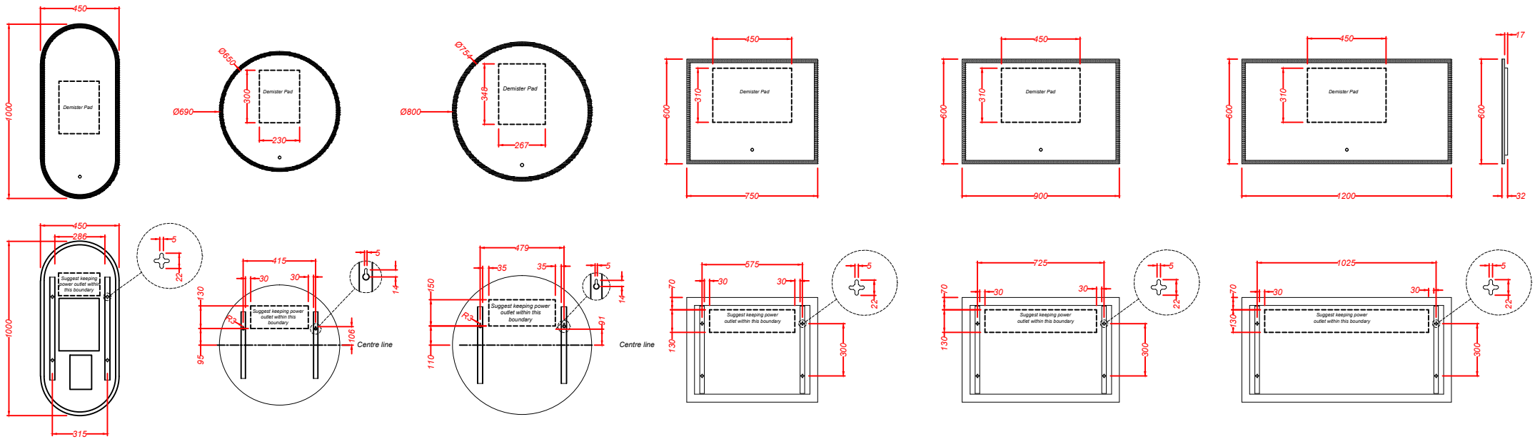
Rear Mounting Details - Use Template provided
