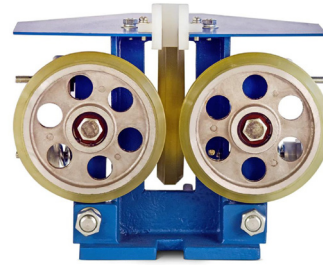
Delco RGA 6" Standard Spring Loaded with Stop Kit and Dust Cover
