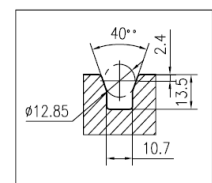
All dimensions are in mm [Inches]
