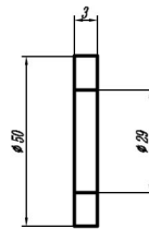
(3) M30 Washer
