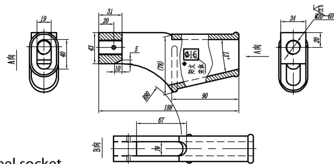
(7) Cast steel socket
