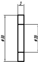
(3) M30 Washer
