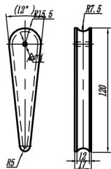
(8) 1/2" (Ø13) Wedge
