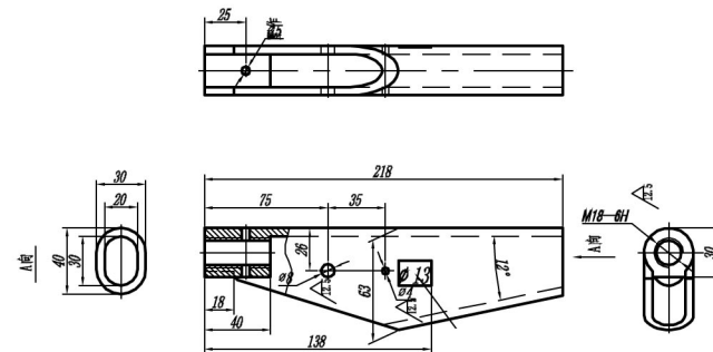
(7) Cast steel socket
