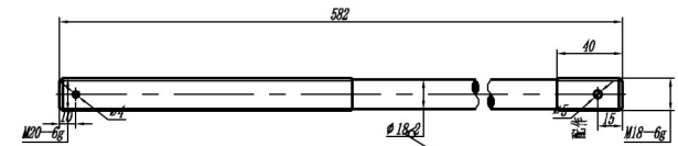
(6) M20 threaded shaft
