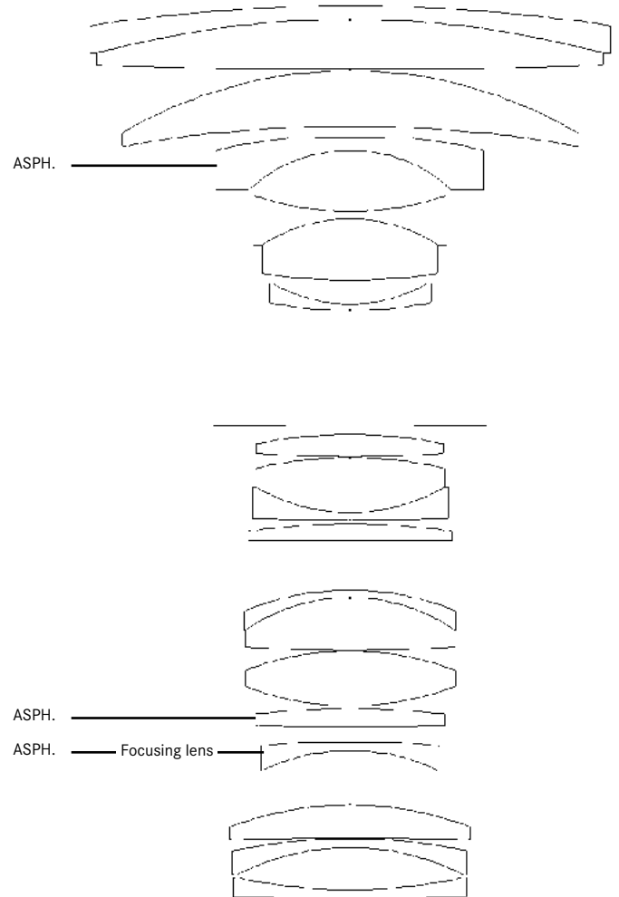
LENS CUT
