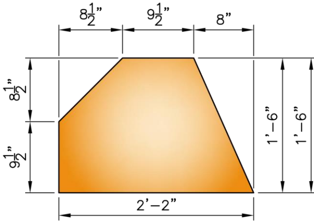
DETAIL ITEM - 1
