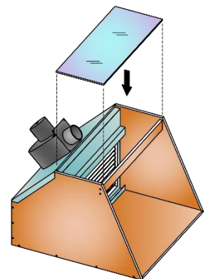
GLASS ASSEMBLING
