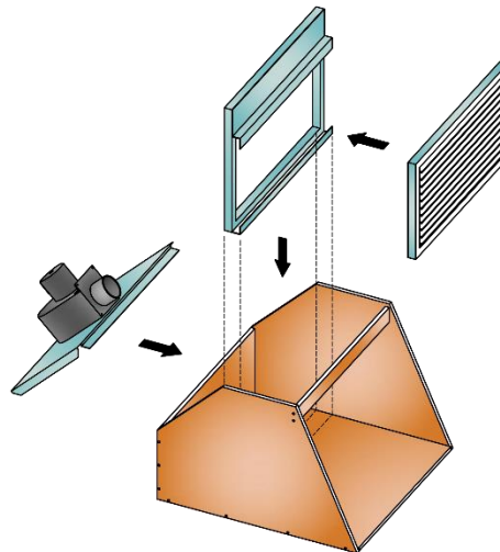
EQUIPMENT ASSEMBLING
