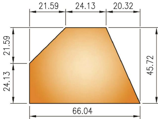
DETAIL ITEM - 1
